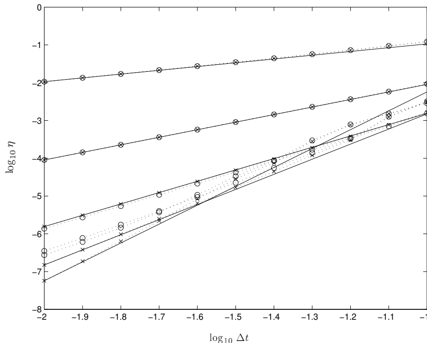
Figure 3: As in Fig. 2: methods \psi_0, \dots, \psi_4 compared for \mathcal{A} = \mathcal{N}_h (crosses) and \mathcal{A} = \mathcal{K}_h (circles) for a nonsymmetric system. Only \mathcal{N}_h has the good order behaviour.
