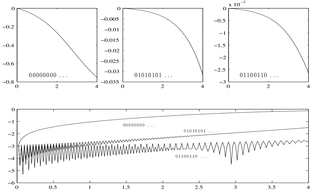
Figure 4: The discrepancy for (4.7) with a step-size \frac{1}{50} . The top figures display the discrepancy for each solution sequence at points m = 2^l , l = 0, 1, 2 , while the bottom figure depicts \log_{10} d(y_n) for the three sequences.
