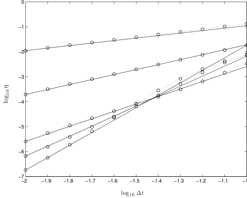
Figure 2: Methods \psi_0 (Euler), \psi_1 = \psi_0 \mathcal{N}_h \psi_0 , \psi_2, \dots, \psi_4 compared for (4.6). Dotted lines connect sample points. Solid lines show predicted slope (symmetry order) of the method, namely \eta (the symmetry error after a fixed time t = 4 ) = \mathcal{O}((\Delta t)^{n+1}) for method \psi_n .
