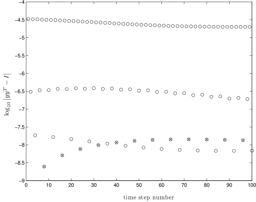
Figure 1: The discrepancy for \psi_3 = \text{'01101001'} applied to Eq. (4.6), where method 0 is \varphi and method 1 is \mathcal{N}_h \varphi . Here \Delta t = \frac{1}{200} . Each eighth step (i.e., a complete cycle) is denoted by a cross.
