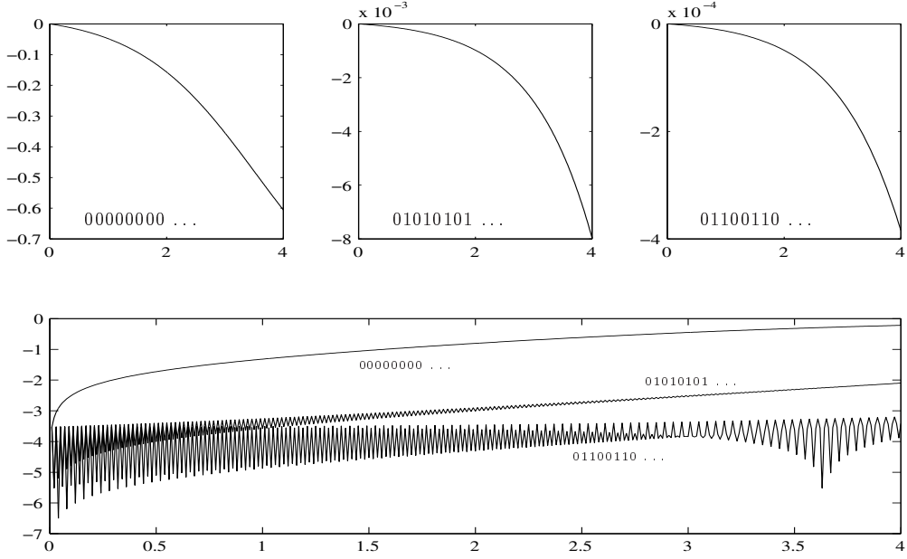
Figure 5: The discrepancy for (4.7) with a step-size \frac{1}{100} . The meaning of different figures is identical to that in Figure 4.
