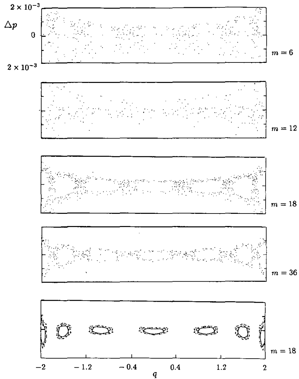
Figure 6. Convergence of a chaotic set. The part of the orbit outlined in figure 5 is magnified for four different numbers, m , of time steps per forcing period. \Delta p is the difference between an iterate of the Poincaré map and the mean orbit (see text). The vertical scale around the mean orbit is expanded by \times 250 . The initial condition is as in figure 5 and 50 000 forcing periods are shown, unless the orbit first drops to a lower level. The bottom picture shows some of the fine structure within the chaotic band.
