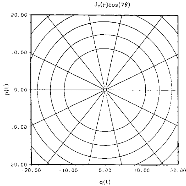
Figure 7. Separatrix mesh. The separatrix mesh for the forced oscillator of section 5.2, calculated from first-order averaging (from Candy and Rozmus (1991)).
