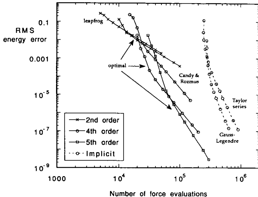
Figure 3. Relative efficiency of different methods. See caption for figure 2. Each implicit method requires two trigonometric function evaluations per iteration in this case; we have counted this as two force evaluations.
