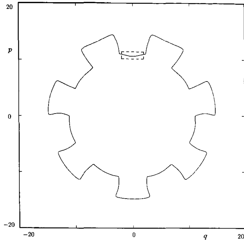
Figure 5. H = \frac{1}{2}(p^2 + q^2) - \epsilon \cos(q - 7t) . Part of an orbit on the chaotic web formed by separatrix splitting (see figure 7). The initial condition is (q_0, p_0) = (0, 10.5939) and there are m = 4 time steps per forcing period. The Poincaré map is shown for 25 000 periods. The orbit stays on the same two separatrix levels.
