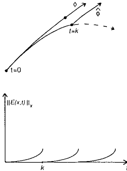
Figure 1. Real and approximate flows. \phi is the flow of the Hamiltonian H ; \hat{\phi} is the flow of the approximate Hamiltonian \hat{H} . E = H - \hat{H} is \mathcal{O}(k^p) , k -periodic, and zero at t = nk .
