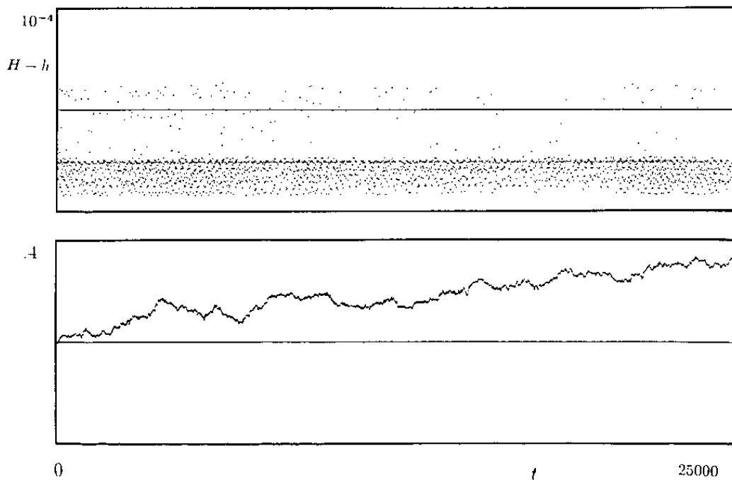
Figure 8. Energy error for coupled pendula. H - h is the change in energy from that at the initial condition, k = 0.5 : (a) initial condition (0, 2) (near elliptic periodic orbit); (b) initial condition (2, 2) (chaotic orbit). Note the different vertical scales.
