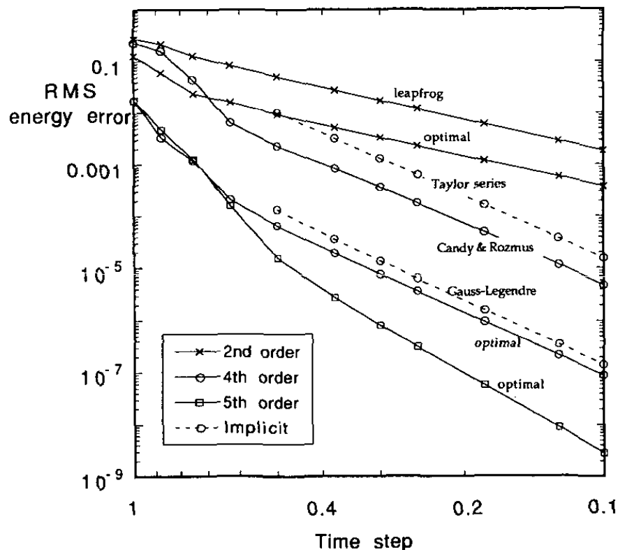
Figure 2. Energy error. The pendulum is integrated up to t = 5000 with initial condition (q, p) = (0, 2) and calculated the root-mean-square energy error over all time steps.
