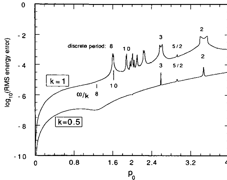
Figure 4. Effect of time step resonances. Here we integrate the pendulum with the optimal fourth-order method for initial conditions (0, p) , 0 < p < 4 . The RMS energy error up to t = 2000 is shown.
