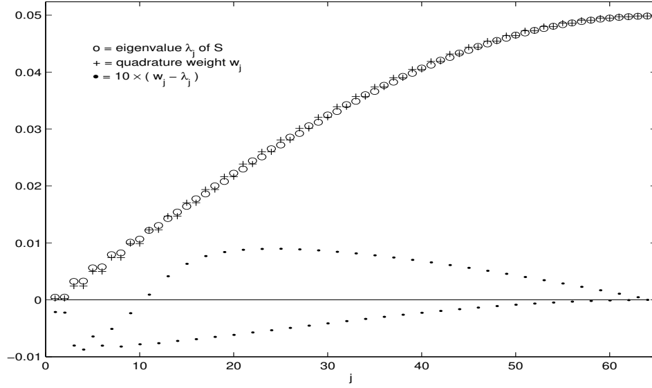
Figure 3: Eigenvalues \lambda_j of the Chebyshev inner product matrix S compared to the Chebyshev quadrature weights w_j , for n = 63 . Also shown are the differences w_j - \lambda_j (magnified ten times).
