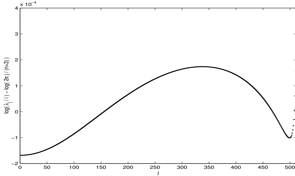
Figure 2: Logarithms of the ratios of the non-zero eigenvalues \pm i\lambda_j of the Chebyshev differentiation matrix factor A , and of 2\pi ij/(n+3) , for n = 1023 (non-zero eigenvalues, which appear to be single and purely imaginary, come in conjugate pairs). All the ratios are very close to 1, which supports Eq. (16). The corresponding graph for n = 1022 , using Eq. (17) instead of Eq. (16), is a carbon copy.
