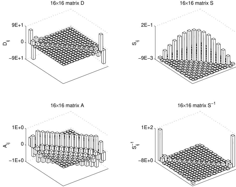
Figure 1: Matrix entries of the Chebyshev differentiation matrix D and its factors S , A and S^{-1} ( D = S^{-1}A ), for n = 15 .
