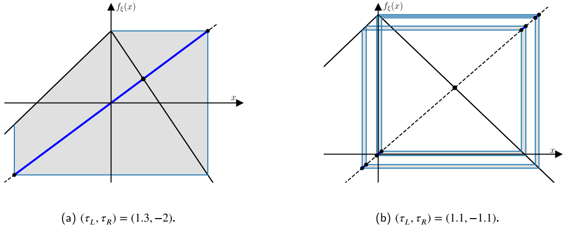
Fig. 1. Cobweb diagrams showing the attractor of the skew tent map (2) with two different combinations of the parameter values. In (a) the attractor is an interval; in (b) the attractor is the union of four disjoint intervals. The maps are also instances of the BCNF (1) with \xi = (1.3, 0, -2, 0) in panel (a) and \xi = (1.1, 0, -1.1, 0) in panel (b).
