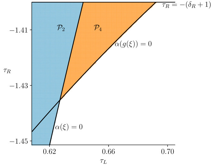
Fig. 17. A magnified version of Fig. 16-b showing the regions having a stable LR -cycle (period-two solution) and a stable LRRR -cycle (period-four solution).
