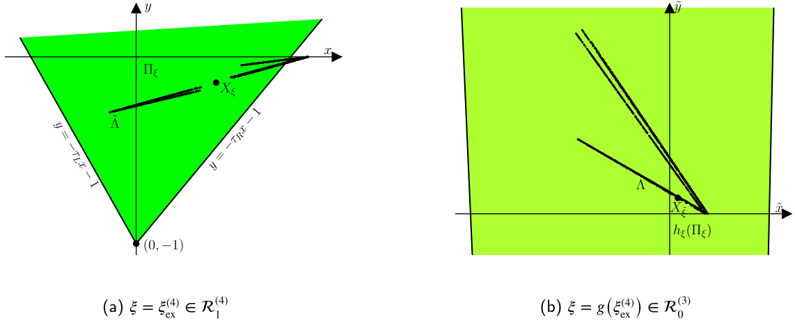
Fig. 18. Panel (a) is a phase portrait of (1) at the parameter point \xi_{\text{ex}}^{(4)} (41) where the attractor has two connected components in the \delta_L < 0 non-invertible case. Panel (b) uses instead g(\xi_{\text{ex}}^{(4)}) .
