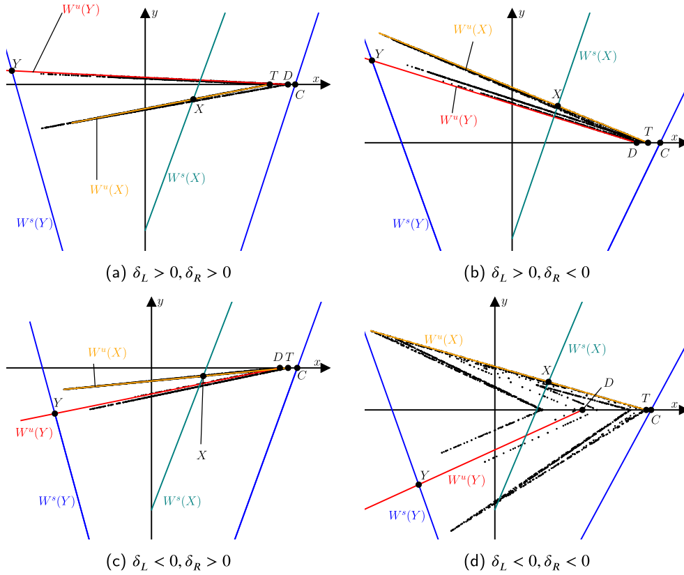
Fig. 3. Phase portraits of the BCNF (1) for four different parameter combinations: (a) \xi = (2.1, 0.06, -1.7, 0.18) ; (b) \xi = (2.1, 0.4, -1.7, -0.55) ; (c) \xi = (2.2, -0.3, -1.7, 0.1) ; (d) \xi = (1.8, -0.75, -1.6, -0.4) . Each plot shows the linear segments of the stable and unstable manifolds emanating from the fixed points X and Y , as well as an adjoining segment of the stable manifold of Y . We also indicate some of their intersections with y = 0 : T , D , and C ; formulas for these are given by (11), (12), and (13). To illustrate the chaotic attractor the black dots show 2000 iterates of a typical forward orbit after transient dynamics has decayed.
