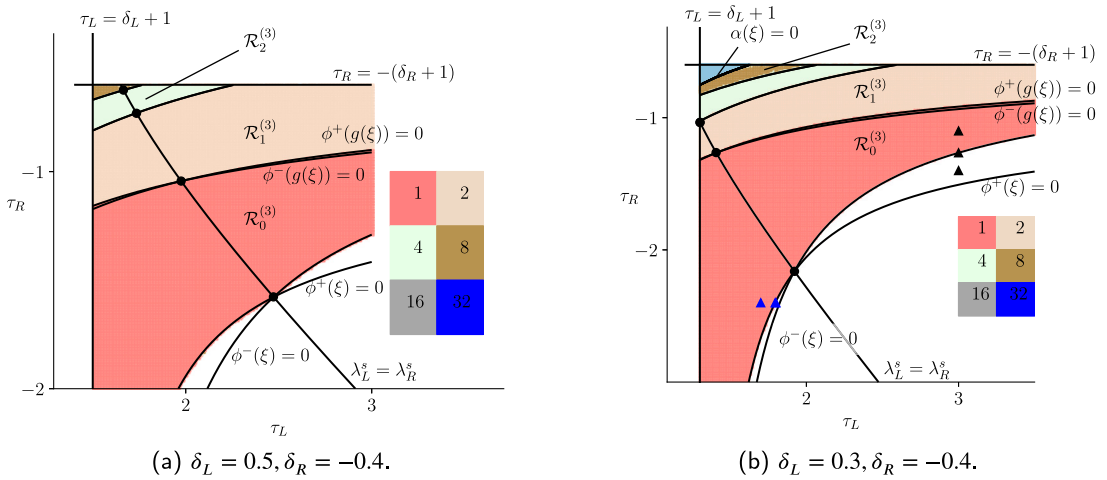
Fig. 12. Two-dimensional slices of the non-invertible parameter region \Phi^{(3)} showing the bifurcation curves overlaid upon numerical results obtained using \varepsilon = 0.001 and M = 10^6 . The blue [black] triangles correspond to the parameter values of Fig. 10 [Fig. 11].
