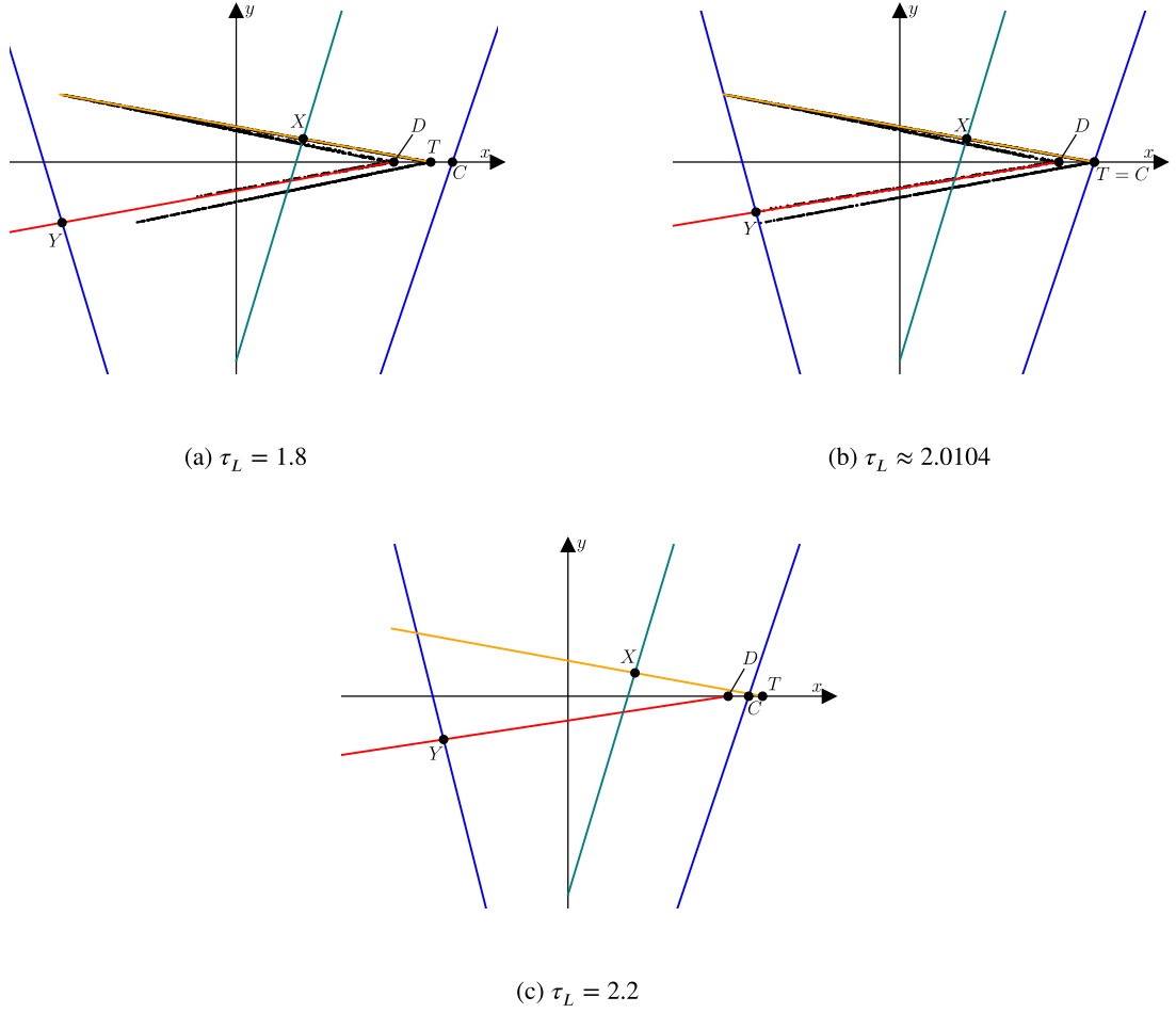
Fig. 7. Phase portraits of Eq. (1) with \delta_L = -0.2 , \delta_R = -0.2 , \tau_R = -1.8 , and three different values of \tau_L corresponding to the black triangles in Fig. 8-b. Panel (b) uses \tau_L such that \phi^-(\xi) = 0 to ten decimal places. In (a) \text{cl}(W^u(X)) is a chaotic attractor; in (b) W^u(X) and W^s(Y) have corner intersections; in (c) there is no attractor.
