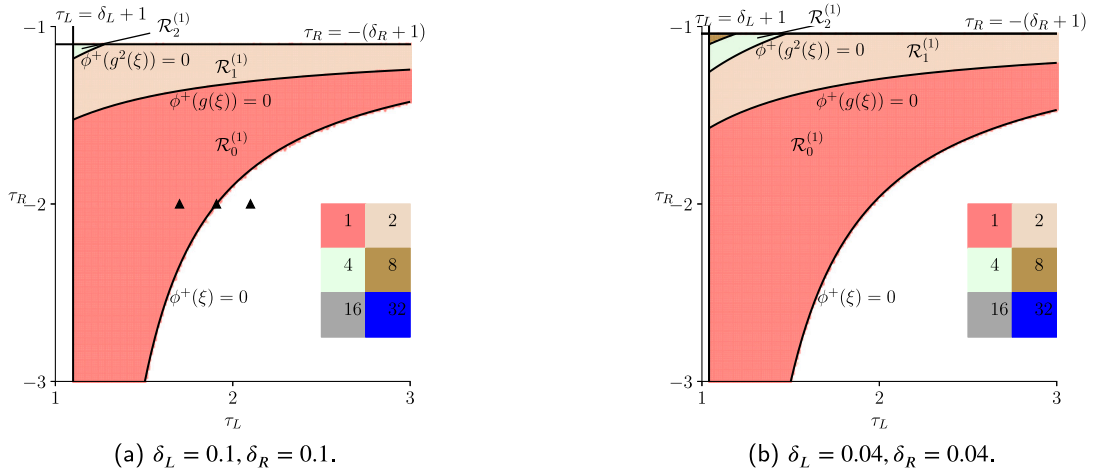
Fig. 6. Two-dimensional slices of the orientation-preserving parameter region \Phi^{(1)} showing the curves \phi(g^n(\xi)) = 0 , for low values of n , overlaid upon the numerical results of Eckstein's greatest common divisor algorithm, explained in Section 6. Each point in a 200 \times 200 grid is coloured by the greatest common divisor of a set of close return iteration numbers J according to the colour bar on the right. In the algorithm we used \varepsilon = 0.001 and M = 10^6 ; also points are coloured white if iterates appeared to diverge. The black triangles correspond to the parameter values of Fig. 5.
