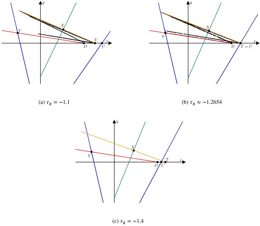
Fig. 11. Phase portraits of (1) with \delta_L = 0.3 , \delta_R = -0.4 , \tau_L = 3 , and three different values of \tau_R corresponding to the black triangles in Fig. 12-b.
