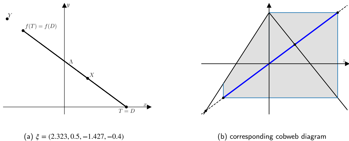
Fig. 19. Panel (a) shows the attractor of (1) at the given parameter point which belongs to \mathcal{R}_0^{(3)} . This attractor is the line segment from T to f_\xi(T) . The restriction of f_\xi to the attractor is the one-dimensional map (43) indicated in panel (b).
