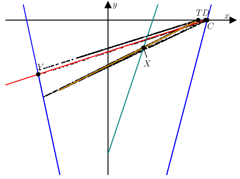
(b) \tau_L \approx 2.2285
