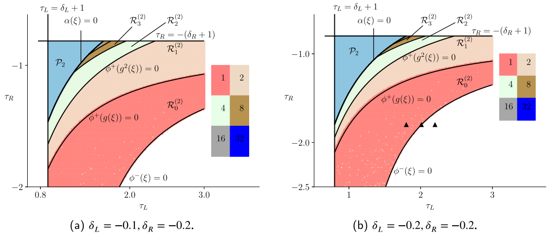
Fig. 8. Two-dimensional slices of the orientation-reversing parameter region \Phi^{(2)} showing the bifurcation curves overlaid upon numerical results obtained using \varepsilon = 0.0001 and M = 10^6 . The black triangles correspond to the parameter values of Fig. 7.
