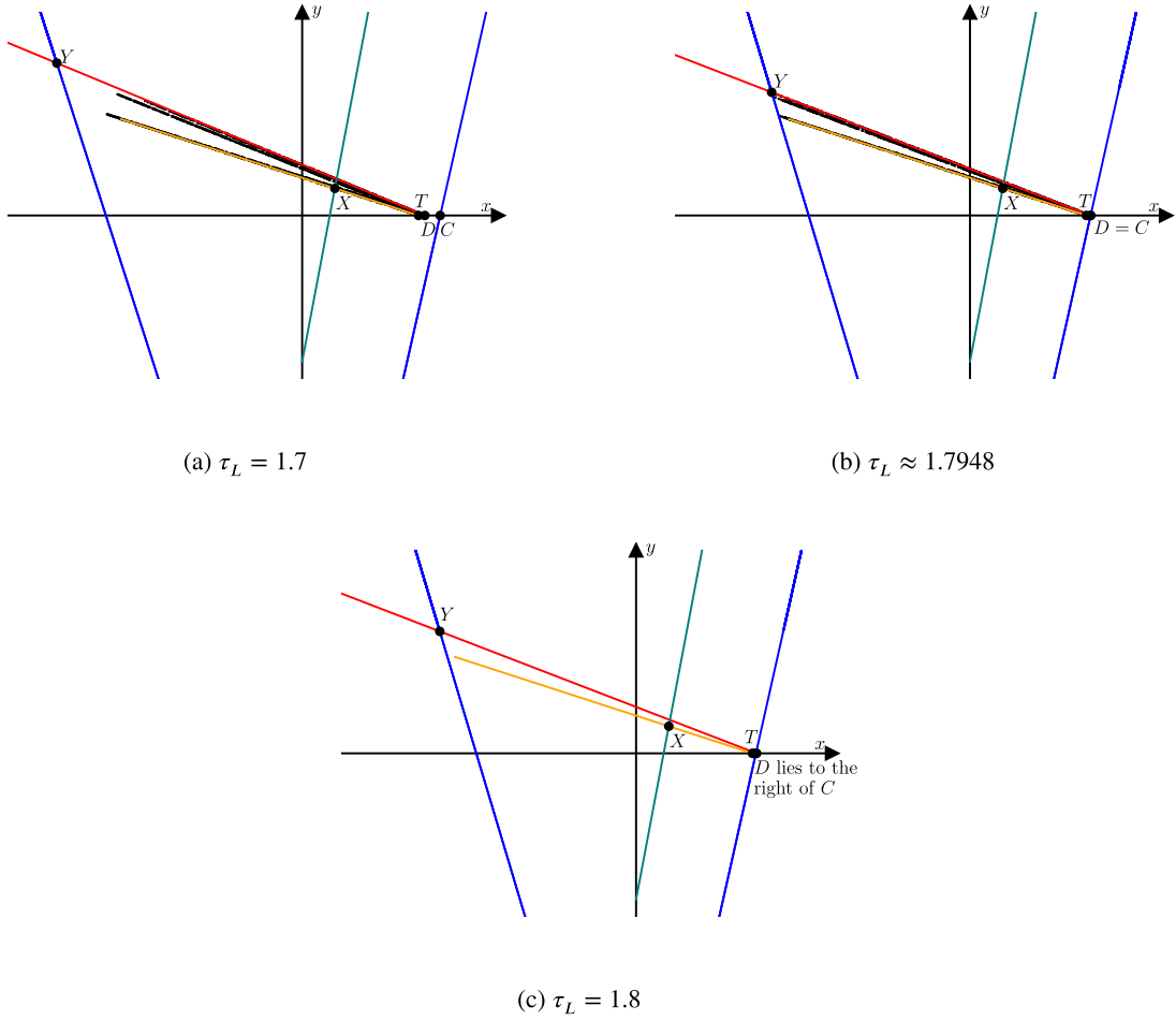
Fig. 10. Phase portraits of (1) with \delta_L = 0.3 , \delta_R = -0.4 , \tau_R = -2.4 and three different values of \tau_L corresponding to the blue triangles in Fig. 12-b.
