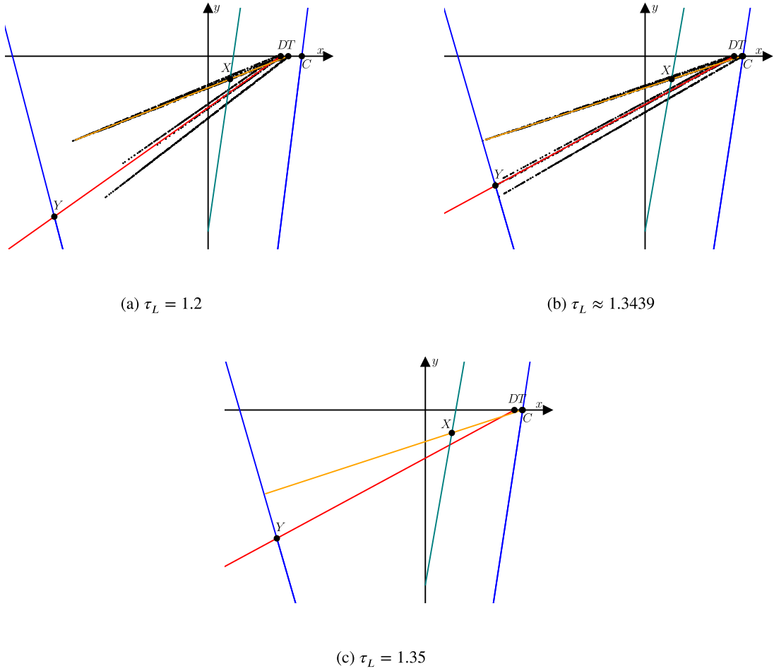
Fig. 14. Phase portraits of (1) with \delta_L = -0.4 , \delta_R = 0.4 , \tau_R = -2.8 , and three different values of \tau_L corresponding to the blue triangles in Fig. 16-a. The parameter value used in panel (b) is approximately where the attractor is destroyed. In all three panels D lies to the left of T which lies to the left of C .
