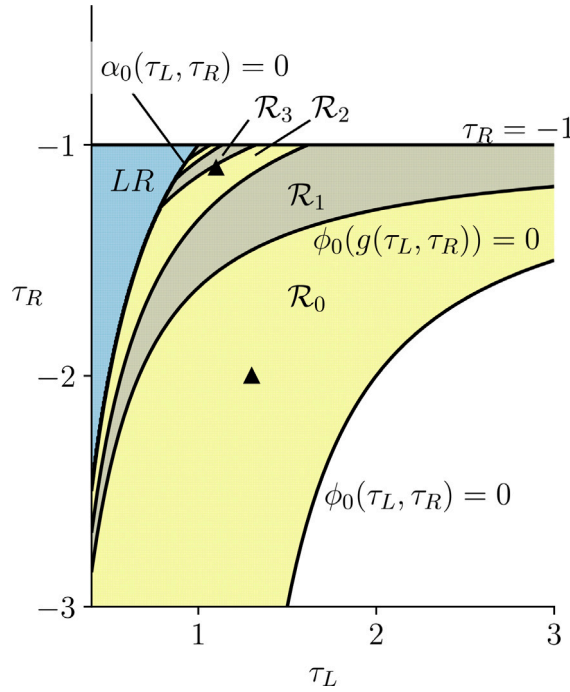
Fig. 2. A two-parameter bifurcation diagram of the skew tent map family (2). In \mathcal{R}_0 the attractor is an interval. In each \mathcal{R}_n with n \geq 1 the attractor is comprised of 2^n disjoint intervals. Below \phi_0(\tau_L, \tau_R) = 0 the map has no attractor; above \tau_R = -1 it has a stable fixed point in x > 0 ; in the top-left region it has a stable LR -cycle (period-two solution). The triangles indicate the parameter values used in Fig. 1.
