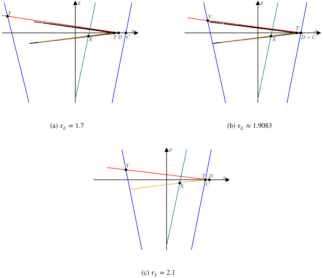
Fig. 5. Phase portraits of (1) with \delta_L = 0.1 , \delta_R = 0.1 , \tau_R = -2 and three different values of \tau_L . These parameter values correspond to the black triangles in Fig. 6-a. Panel (b) uses \tau_L such that \phi^*(\xi) = 0 to ten decimal places. In (a) \text{cl}(W^u(X)) is a chaotic attractor; in (b) W^s(Y) and W^u(Y) form a homoclinic corner by intersecting at D = C ; in (c) there is no attractor.
