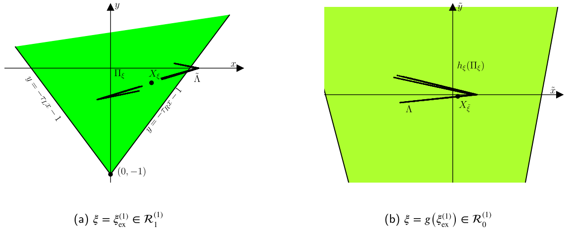
Fig. 4. Phase portraits of the BCNF (1). Panel (a) uses the example parameter point \xi_{\text{ex}}^{(1)} given by (20) where the attractor \tilde{\Lambda} has two connected components, one of which lies entirely in \Pi_\xi (shaded). Panel (b) uses the parameter point g(\xi_{\text{ex}}^{(1)}) where the attractor \Lambda has one connected component in h_\xi(\Pi_\xi) (shaded).
