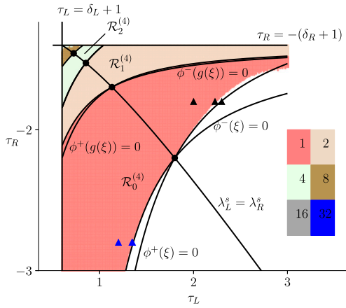
(a) \delta_L = -0.4, \delta_R = 0.4 .
