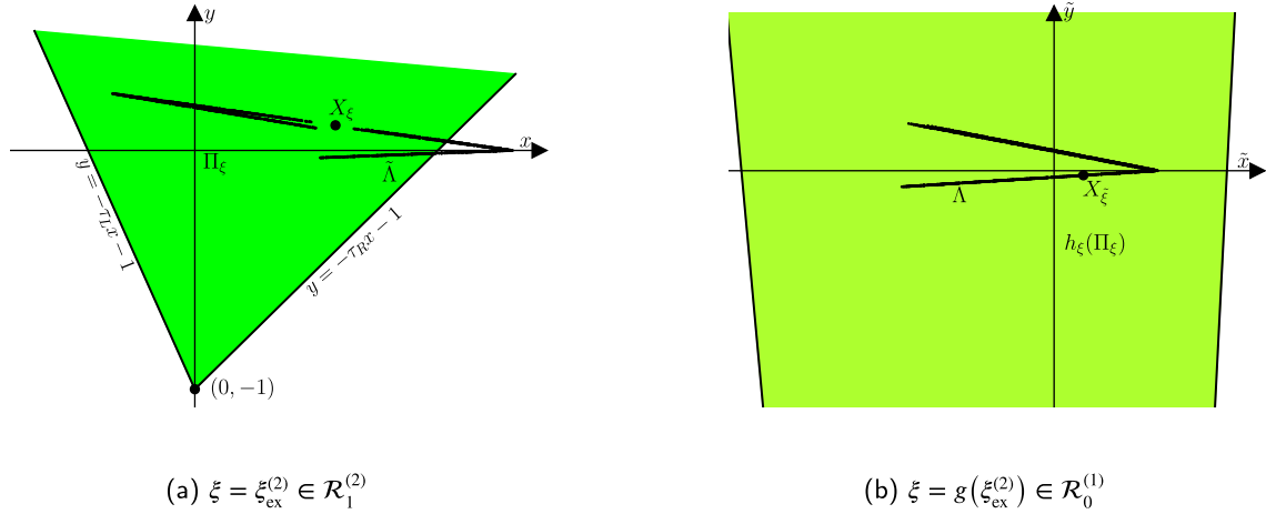
Fig. 9. Panel (a) is a phase portrait of (1) at the parameter point \xi_{\text{ex}}^{(2)} (33) where the attractor has two connected components in the orientation-reversing case. Panel (b) uses instead g(\xi_{\text{ex}}^{(2)}) .
