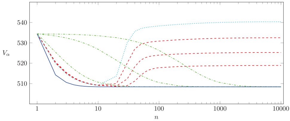
Figure 3. TV deblurring functional Baboon, explicit Euler method with step size \tau = 0.19 (cyan dotted line), explicit Euler with \tau = 0.185, 0.18, 0.175 (red dashed lines, top to bottom), explicit Euler with \tau = 0.1, 0.01, 0.001 (green dash-dotted lines, left to right), discrete gradient method (blue solid line) with step size \tau = 2.5 (in all experiments: \alpha = 0.05, \beta = 0.001 ).
