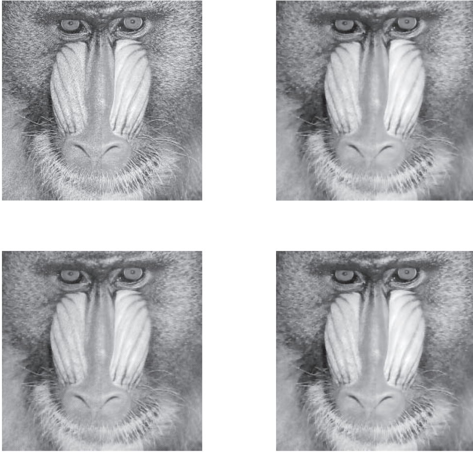
Figure 2. Noisy baboon picture (top left) and TV -denoised reference picture with the explicit Euler method, step-size \tau = 0.001 after 10 000 steps (top right), explicit Euler denoised image with step-size \tau = 0.3 after 10 000 steps (bottom left) and discrete gradient denoised baboon with step-size \tau = 2.5 after 10 steps (bottom right).
