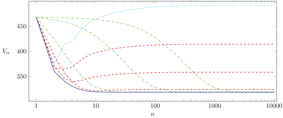
Figure 1. TV functional Baboon, explicit Euler method with step size \tau = 0.5 (cyan dotted line), explicit Euler method with \tau = 0.4, 0.3, 0.2 (red dashed lines, top to bottom), explicit Euler with \tau = 0.1, 0.01, 0.001 (green dash-dotted lines, left to right) discrete gradient method (blue) with step size \tau = 2.5 (in all experiments: \alpha = 0.05 , \beta = 0.001 ).
