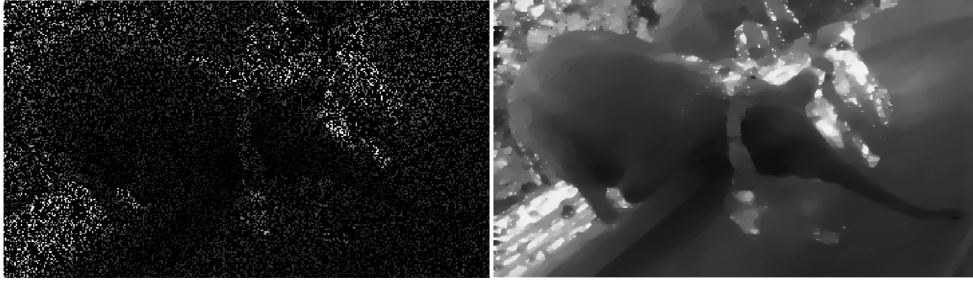
Figure 5. Given image with 80% of all pixels missing and TV -inpainting image with DG method and adaptively chosen \tau .
