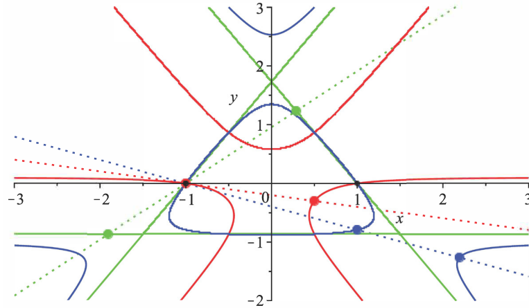
Figure 2. The curves \tilde{H} = \frac{\sqrt{3}}{2} , \tilde{H} = -\frac{1}{10} , \tilde{H} = 1 , in resp. green, red and blue. Here h = 1 .
