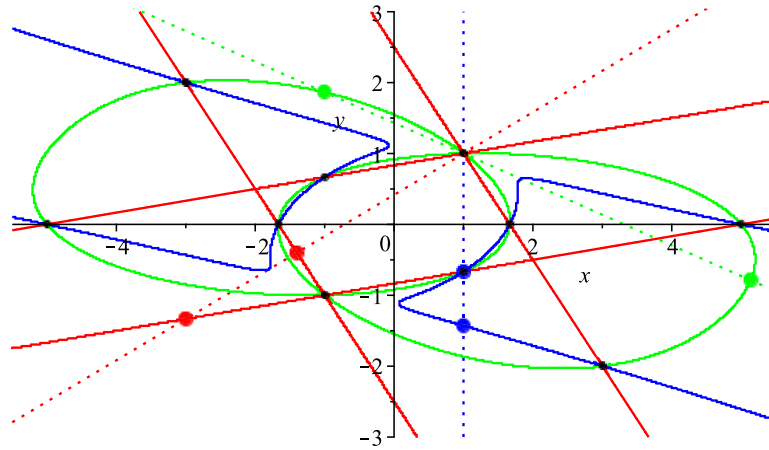
Figure 3. The curves \tilde{H} = 25 , \tilde{H} = \frac{125}{16} , \tilde{H} = -100 , in resp. green, red and blue. Here h = \frac{1}{5} .
