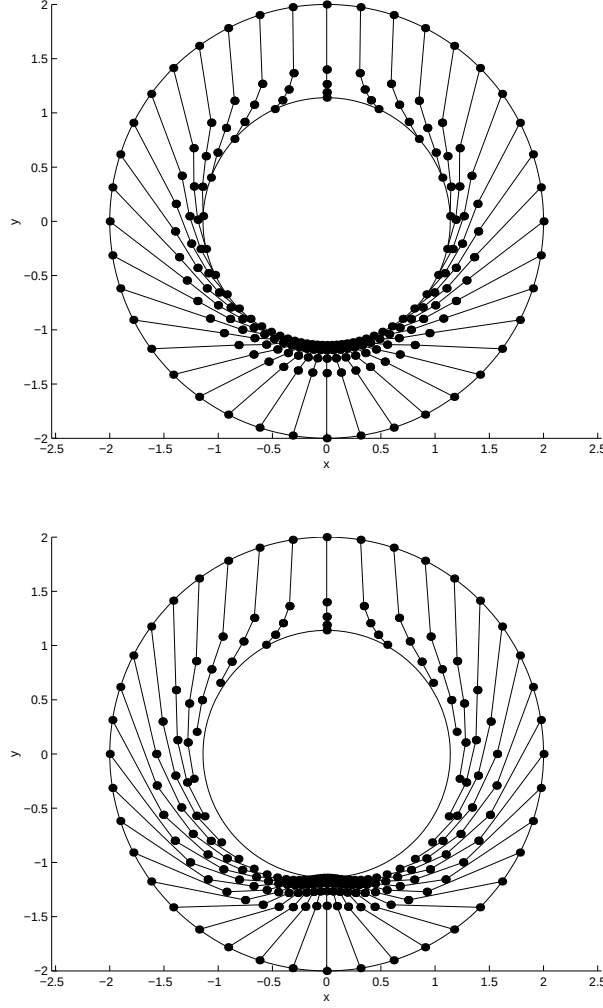
Fig. 2. Foliate vs. nonfoliate integrators. The ODE of Eq. (1) is integrated by the (foliate) Lie-Euler method Eq. (??) (top), and the (nonfoliate) Euler method (bottom). The 20 initial conditions lie on a circle of radius 2, and four time steps of 0.1 are shown. In the nonfoliate integrator, the final values do not lie on the reference circle shown. Note that the two methods coincide on x = 0 , where the tangential component vanishes.
