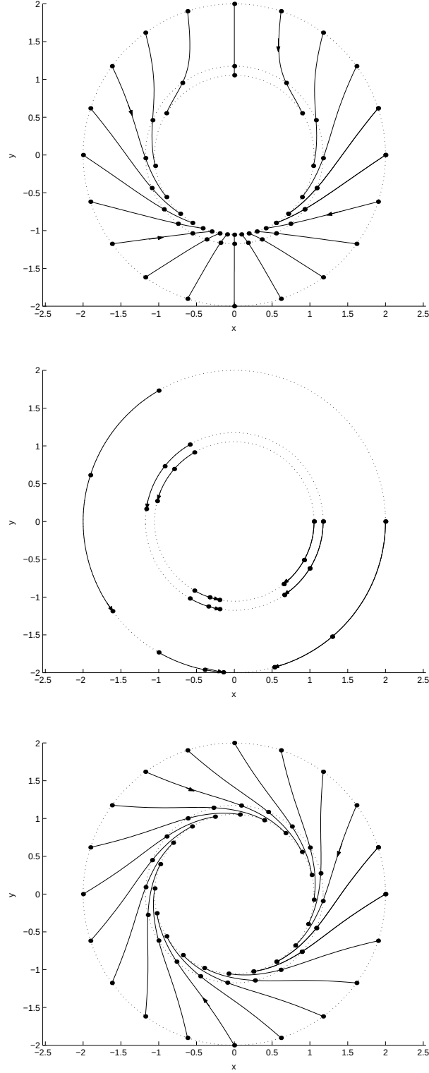
Fig. 1. Three foliate vector fields. Top: a general foliate vector field, \dot{r} = r(1 - r^2) , \dot{\theta} = -r \cos \theta (Eq. (??)). Middle: a system with an integral, \dot{r} = 0 , \dot{\theta} = -r \cos \theta . Bottom: a system with a continuous symmetry, \dot{r} = r(1 - r^2) , \dot{\theta} = -(1 + r^2/5) . All three flows map circles to circles. The dots mark times 0, 0.5, and 1.
